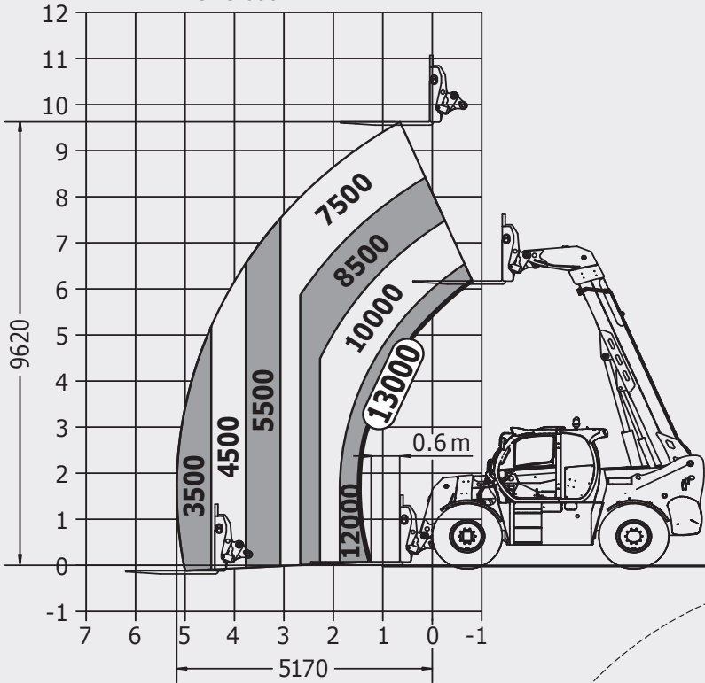
Machine on tyres with forks CDG 600 mm
